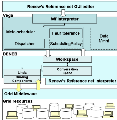
Fig. 3. Vega's architecture and its relationship with other systems
