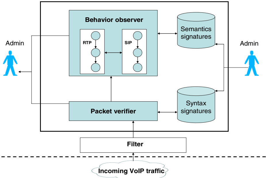
Fig. 3. System Architecture
