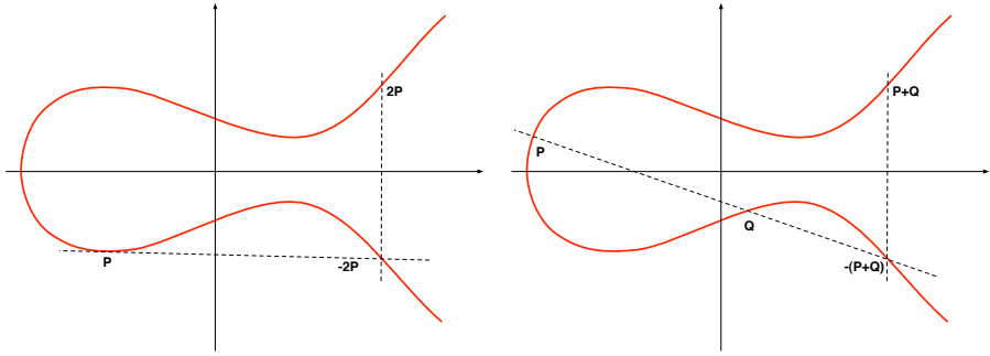
(a) Point doubling.
