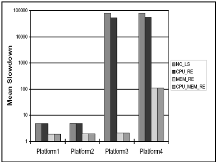
Fig. 3. Mean slowdowns of “trace 0” on different heterogeneous platforms, with mean memory size of 8 Mbytes
