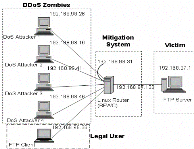
Fig. 3. Experimental environment setup
