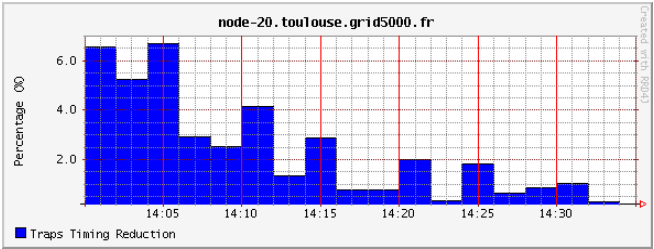
Fig. 10. Auto-configuration Overload
