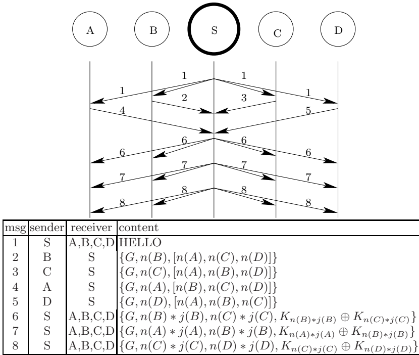
Fig. 5. Cluster key scheme. Sensor nodes A , B , C and D are connected to each other and want to form a cluster key via a mobile node S . The required exchange of messages is similar to the one in Fig.3 with the difference that here the nodes also agree on a cluster identifier G . Thus, when the nodes receive an HELLO message from the mobile node (transmission 1), they send back a key request message that includes the cluster identifier (transmissions 2,3,4,5), their own identifiers and the identifiers of the nodes which were announced to them. After the mobile node receives this information, it broadcasts a chain of reply messages (transmissions 6,7,8). Each of these messages contains the cluster identifier G , the identifiers of two nodes and XOR results of the keys they own. The value of j is not incremented, in other words the key corresponding to a particular node remains the same for all XOR operations carried out by the mobile node.
