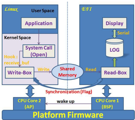
Fig. 3. System Call Monitor
