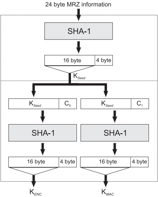
Fig. 2. Basic Access Key Derivation
