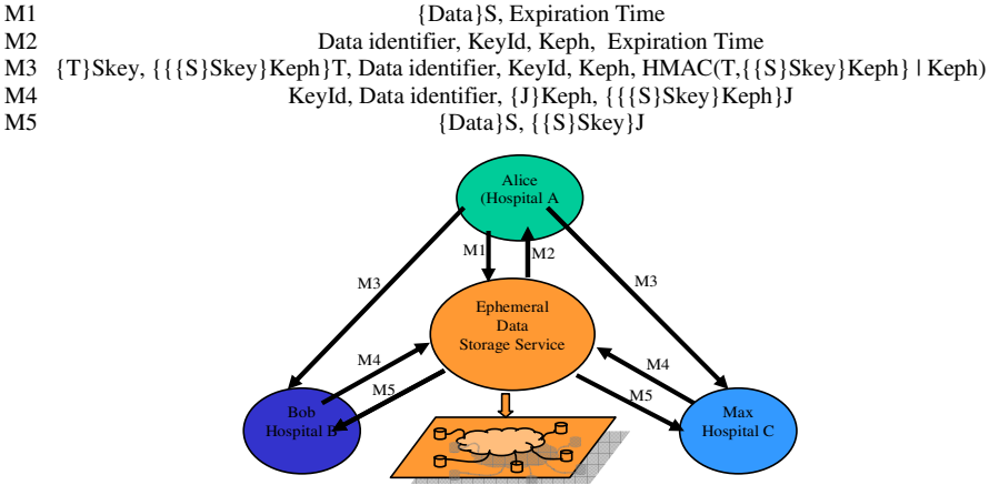
Fig. 4. Implemented Centralized Environment and Protocol
