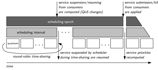
Fig. 3. Two-level scheduling policy
